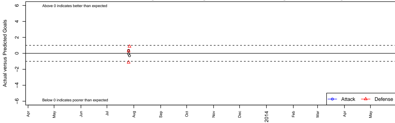
OHSC Rolling Thunder B99 Dots are actual minus expected GF (blue circles) and GA (red triangles). Blue line is smoothed change in attack strength. Red is smoothed change in defense strength.
